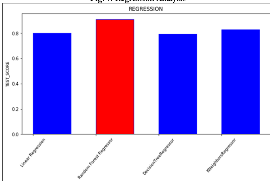
Fig. 7. Regression Analysis
