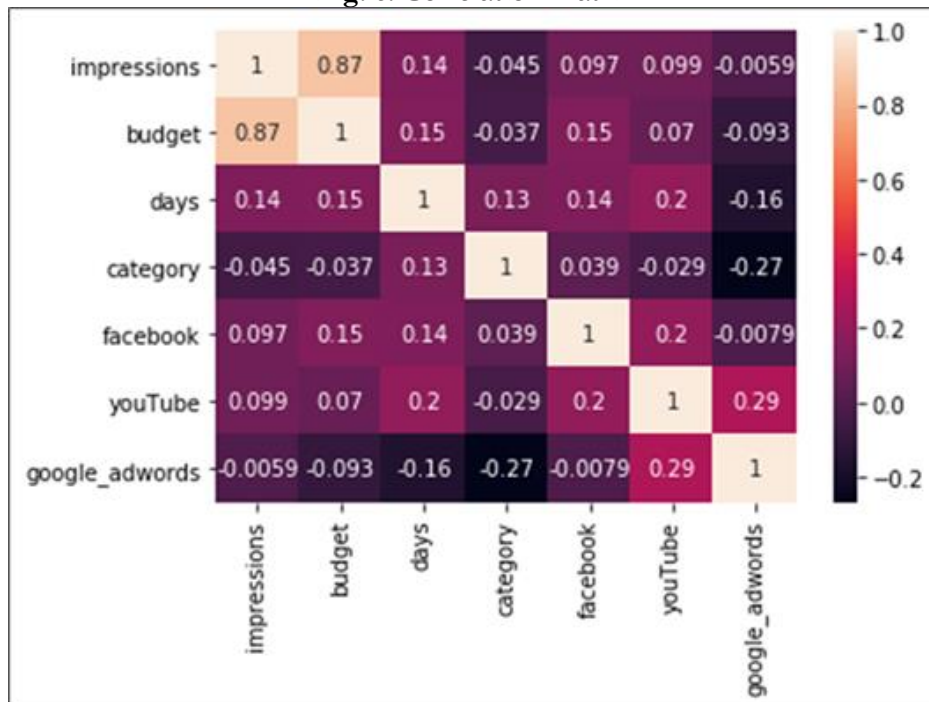
Fig. 6. Correlation Matrix
